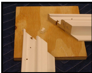
Set Hoffman Key round side up and push top frame down onto the Hoffman Key.
